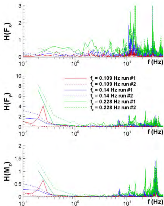
Figure 2-18 Noise test results: FFT for F_x , F_y , and M_z . Groups A shows noise sources from PMM motor, group B shows added noise sources due to motions, and group C shows added noise sources from mechanical vibrations due to carriage speed.
