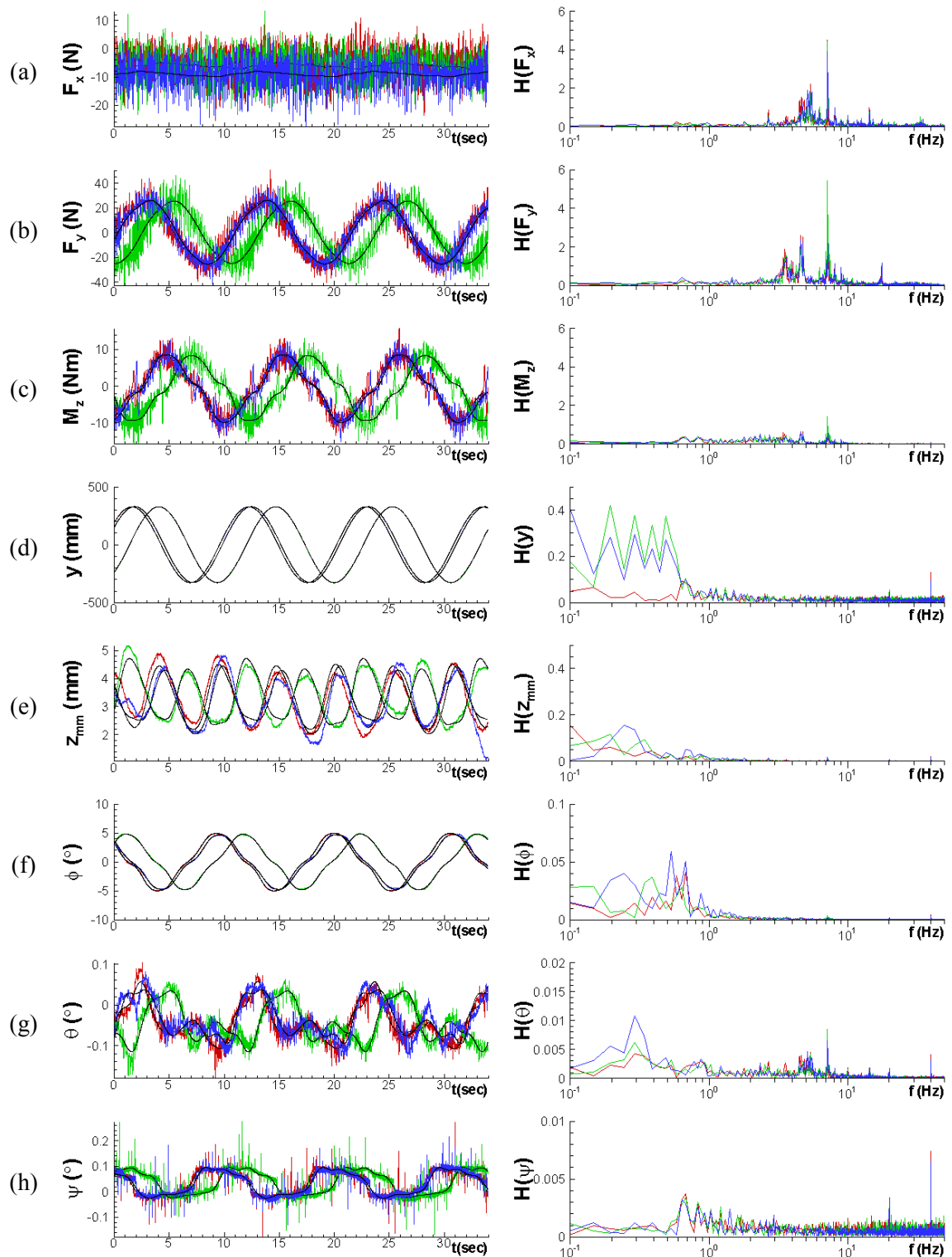
Figure 6-8 Time history (left) and FFT (right) of pure sway test data with Fr = 0.2 and \beta_{max} = 10^\circ : (a) F_x , (b) F_y , (c) M_z , (d) y , (e) z_{mm} , (f) \phi , (g) \theta , and (h) \psi . Colors; red: w/o wind, green: half wind, blue: full wind, black: FS-reconstruction.
