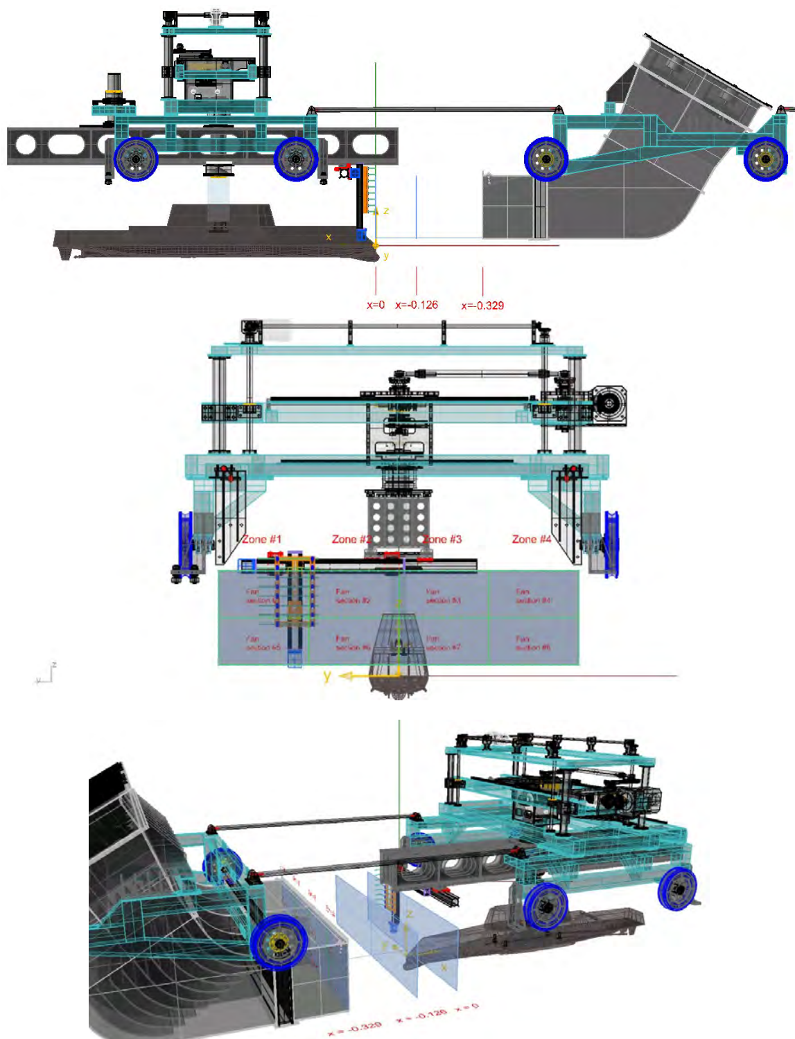
Figure 2-13 Side elevation (top), end view (middle), and perspective (bottom) of carriages, pitot rack, and measurement grid planes. Model and mount are not installed during surveys; just shown for reference. Wind carriage outlet is located at x = -0.33 .
