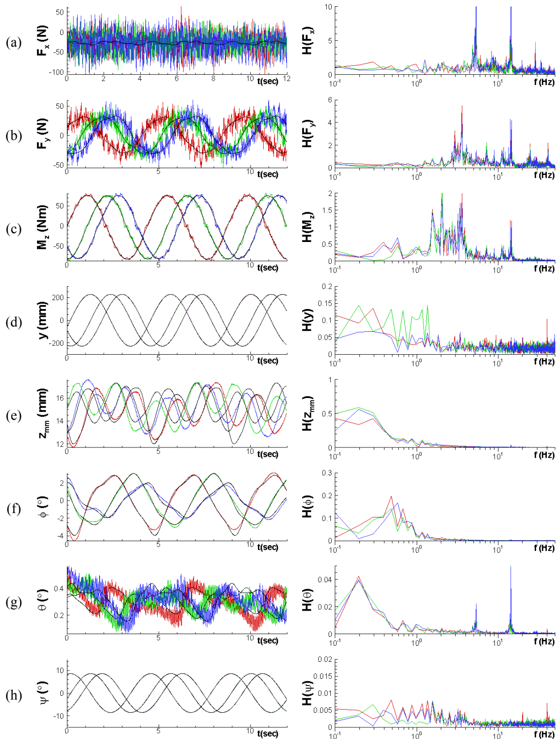
Figure 6-13 Time history (left) and FFT (right) of pure yaw test data with Fr = 0.4 and r_{max} = 0.3 : (a) F_x , (b) F_y , (c) M_z , (d) y , (e) z_{mm} , (f) \phi , (g) \theta , and (h) \psi . Colors: red: w/o wind, green: half wind, blue: full wind, black: FS-reconstruction.
