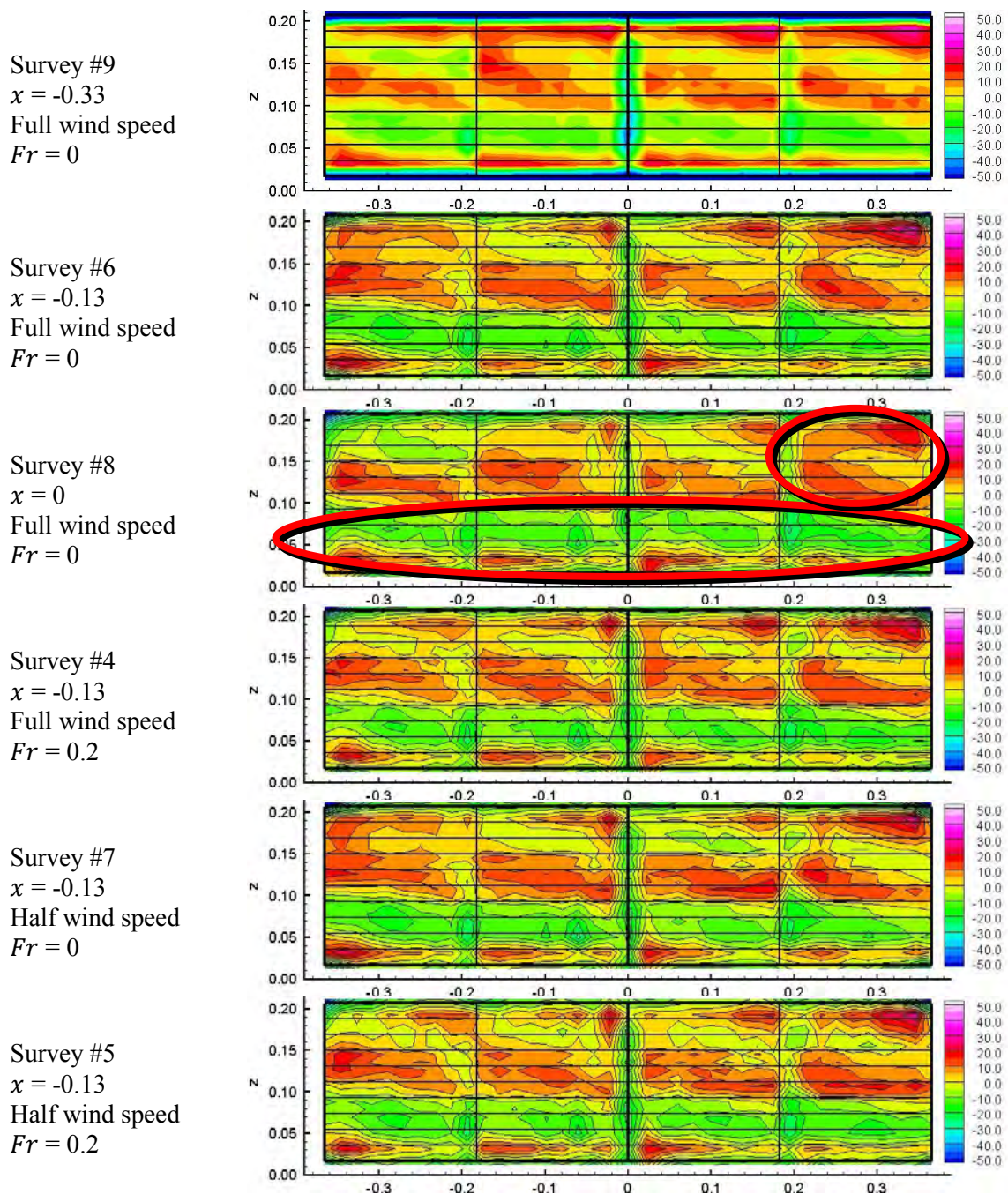
Figure 3-2 Axial velocity data expressed as (\bar{U}_{W_i} - \mu_{\bar{U}_W})/\mu_{\bar{U}_W} (%) for surveys taken before fan and screen adjustments. Medium thick lines represent internal vane locations. Problem areas are circled in red.
