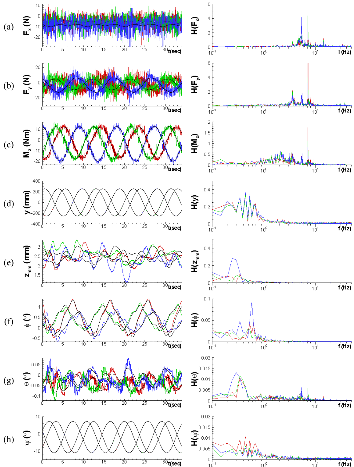
Figure 6-15 Time history (left) and FFT (right) of yaw and drift test data with \beta = -2^\circ : (a) F_x , (b) F_y , (c) M_z , (d) y , (e) z_{mm} , (f) \phi , (g) \theta , and (h) \psi . Colors; red: w/o wind, green: half wind, blue: full wind, black: FS-reconstruction.
